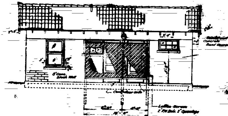
SIDE ELEVATION Scale 1/2" = 1'
